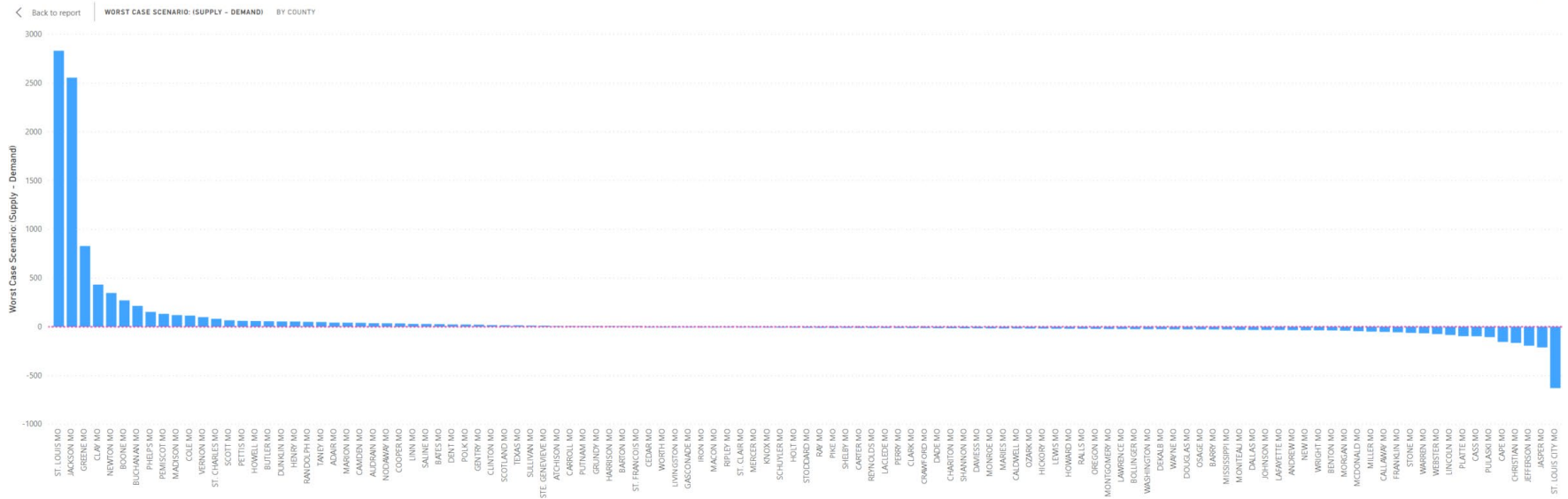
Fig 1: The above figure shows Supply minus Demand at peak using the Imperial-College-COVID19-NPI-modelling-16-03-2020 and the exponential regression model in the article published. All appearing above the red dashed line have capacity even at peak. All Counties that at or falling below the red line are will not be able to meet demand. In this scenario, peak will hit mid-May. Planning for servicing counties that either do not have hospitals or overburdened systems should be made. Some Counties will have capacity to redirect to needed areas.
